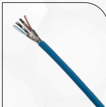
CABLE CAT 6A, 23 AWG, U/UTP, LSZH-1 NUL6X04WH-HEG
